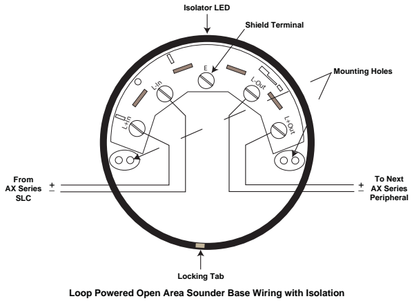
Loop Powered Open Area Sounder Base Wiring with Isolation
