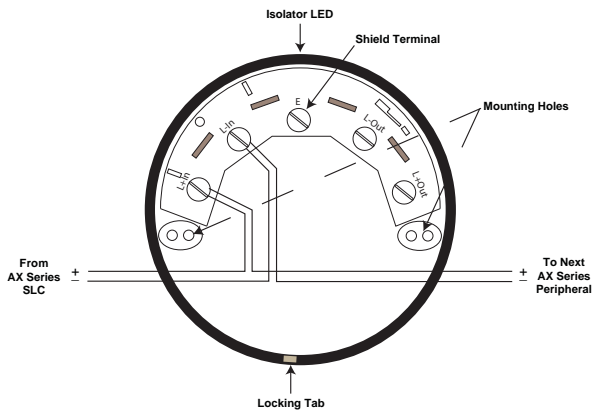
Loop Powered Open Area Sounder Base Wiring without Isolation
